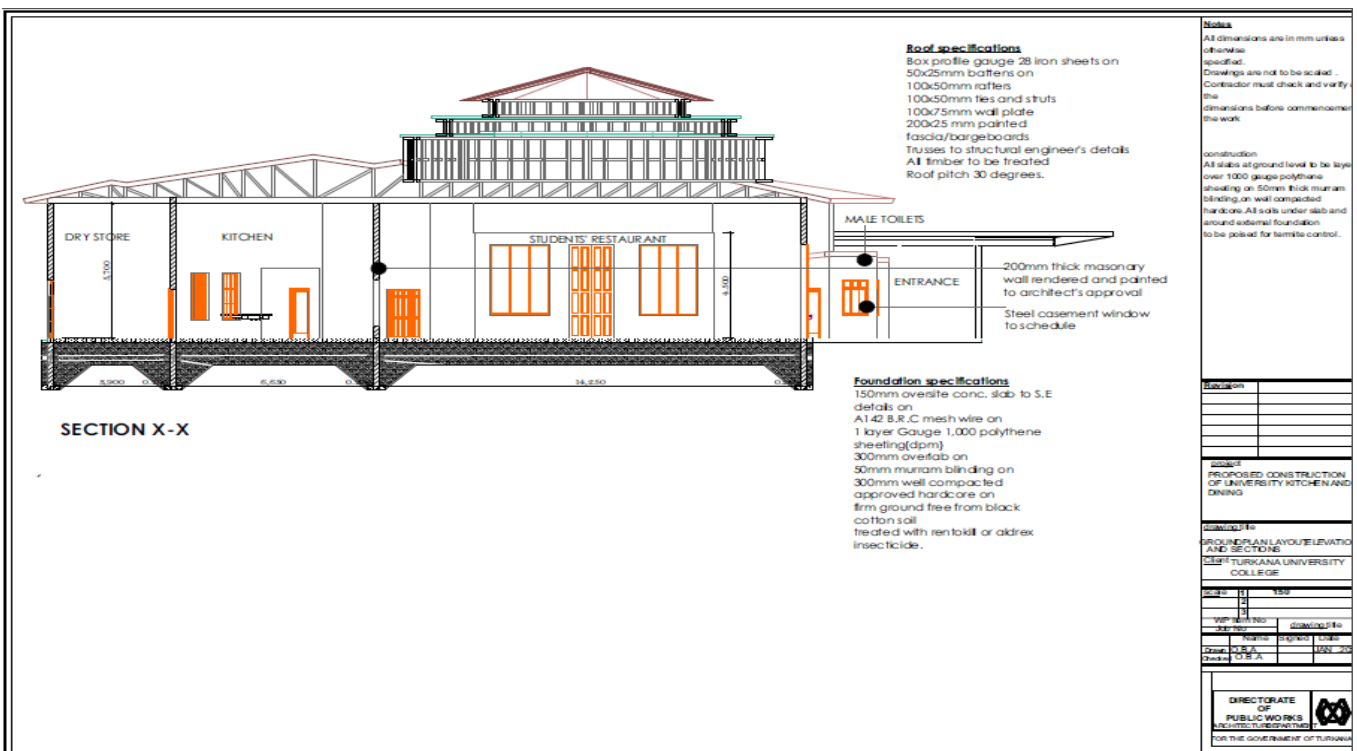
Figure 5: KITCHEN SECTION
