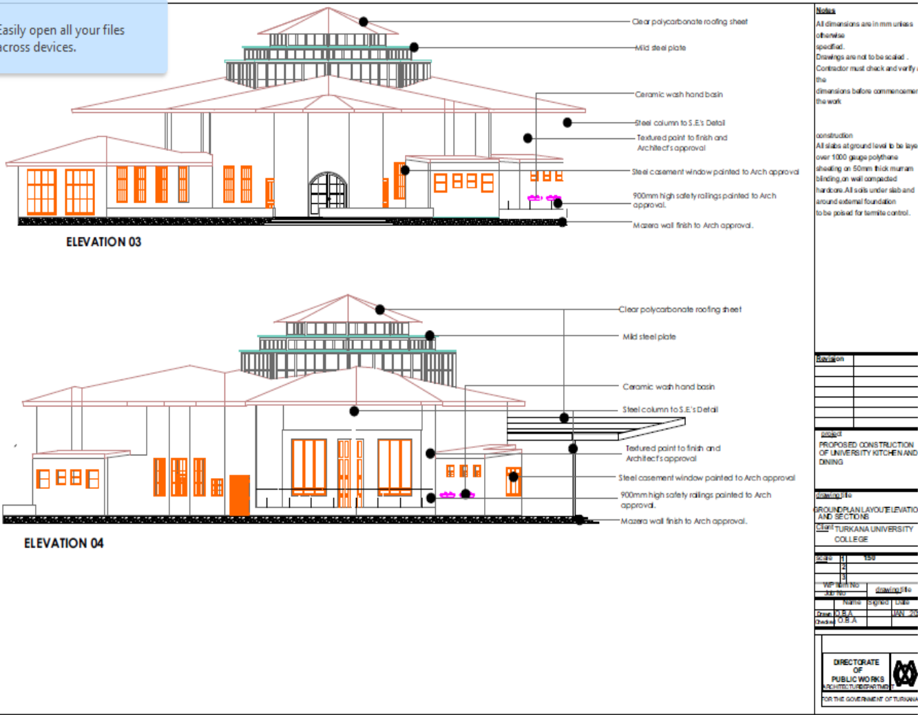
Figure 4: ELEVATIONS
